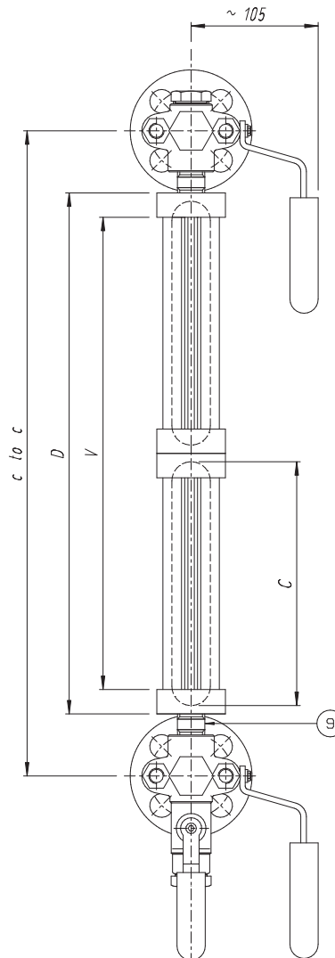
RBB model with NY valves
